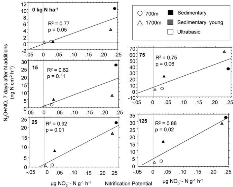
Figure 8. Regression analyses of potential nitrification (prior to N additions) and total soil N-oxide emissions ( N_2O + NO ) seven days after a range of N additions. Note differences in scale between doses of N.
