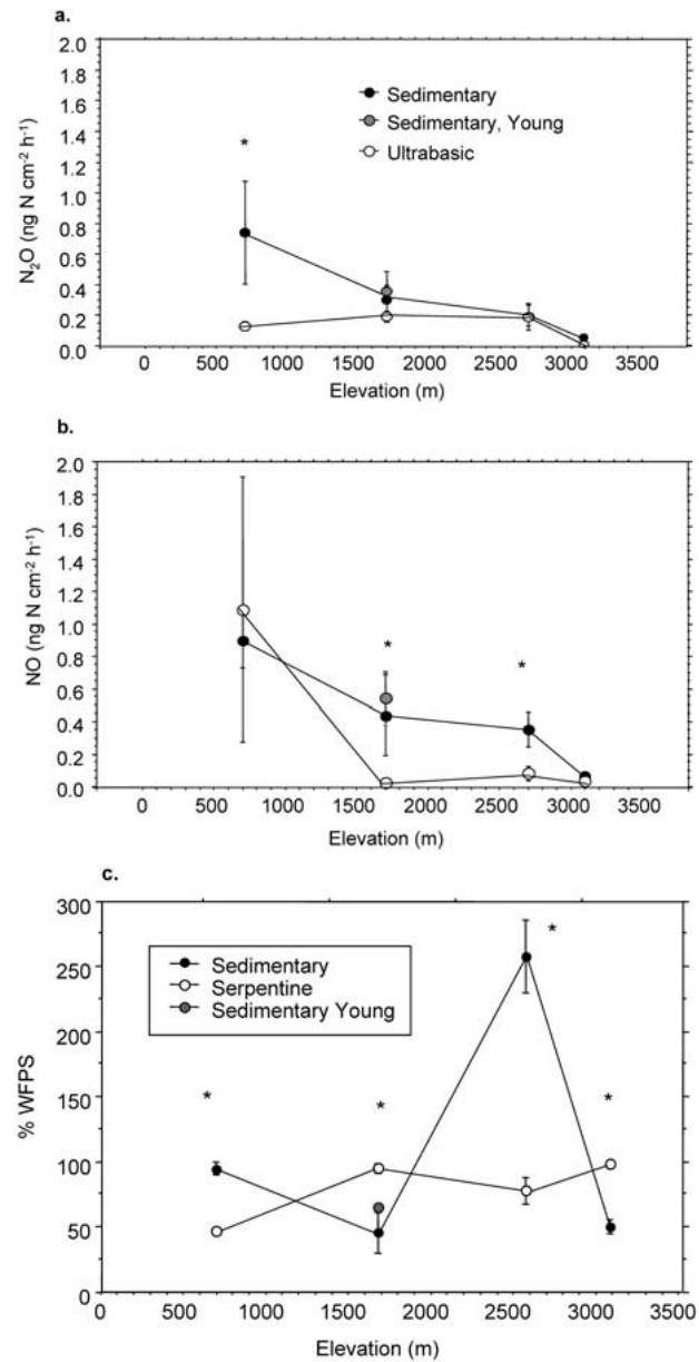
Figure 2. Soil N fluxes and soil properties from primary forest sites on Mt. Kinabalu. (a) N_2O emissions and (b) NO emissions ( \pm SE, n = 6 chambers per site.), and (c) WFPS. Soil cores at each site were taken on subsequent days at the same time as gas measurements over a total of 6 days ( \pm SE, 3 composite samples of 3 cores each, 0–15 cm depth). * Represents significant difference ( p < 0.1 ) between soil types (old substrates only) within an elevation. Sedimentary young site has a substrate age of approximately 35,000 years.
